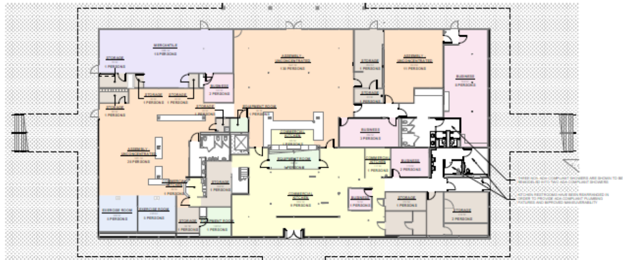
1 FIRST FLOOR PLAN - CODE REVIEW
