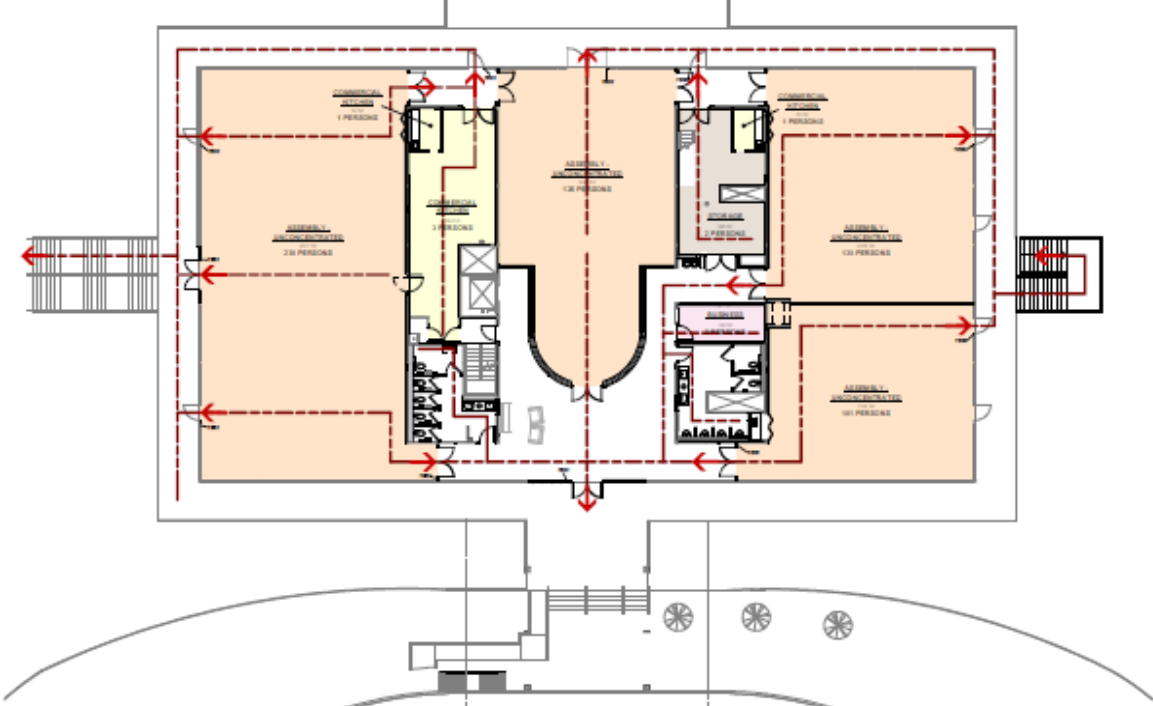
2 SECOND FLOOR PLAN - CODE REVIEW
