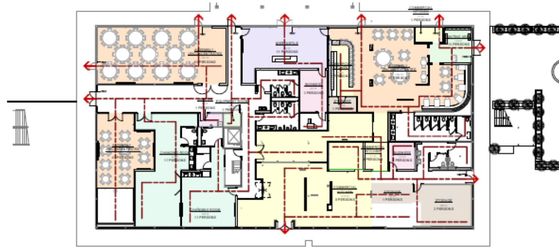
1 FIRST FLOOR PLAN - CODE REVIEW
