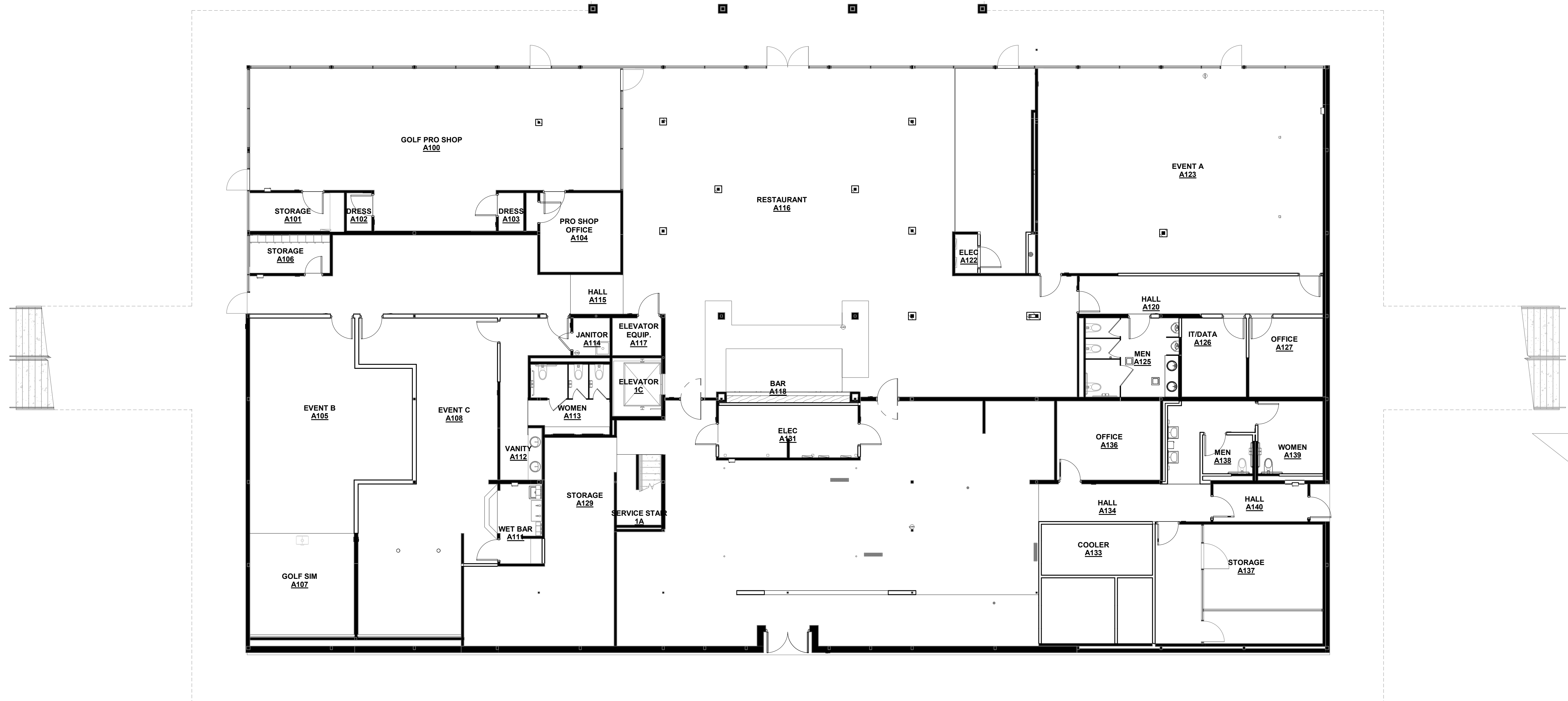
1 FLOOR PLAN - PROPOSED 1/8" = 1'-0" REF: AC500/1
