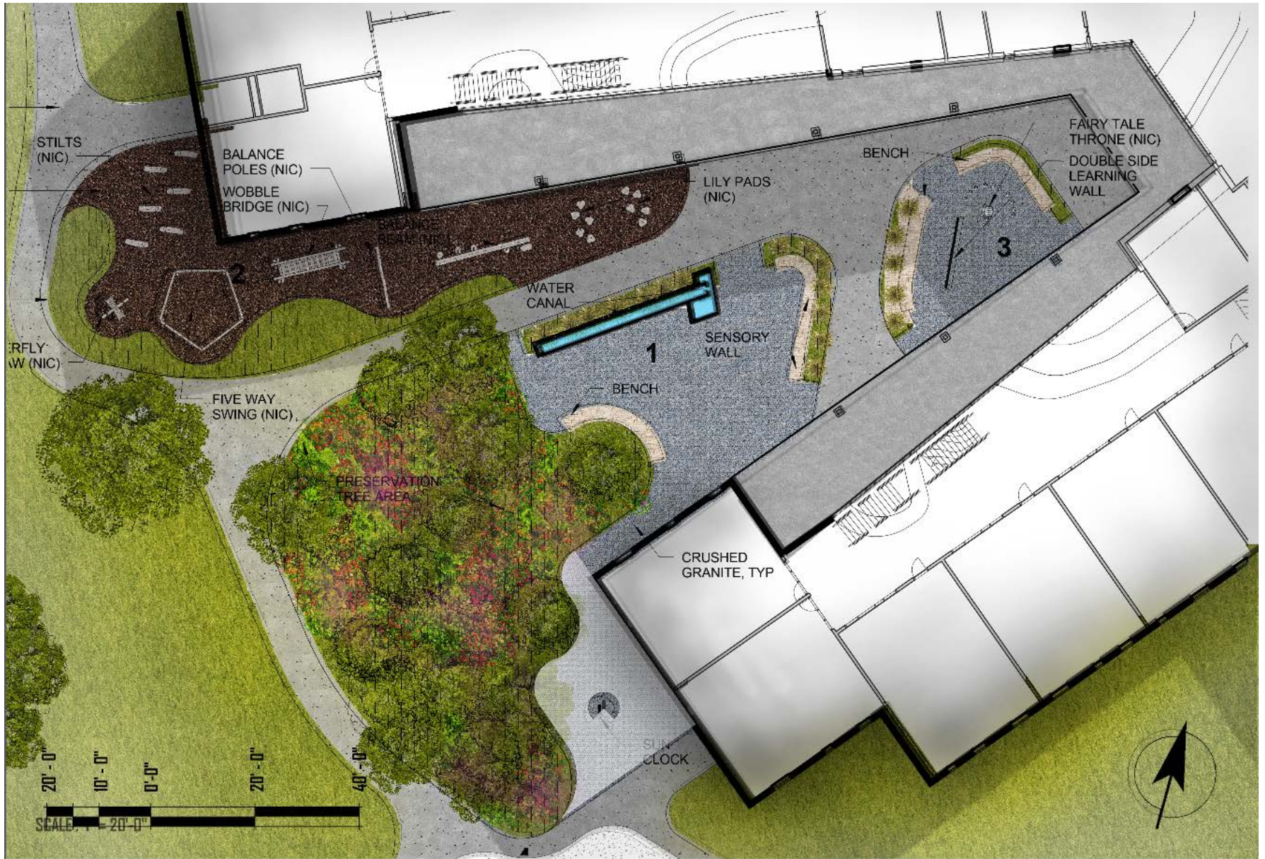
Enlarged Courtyard Plan
